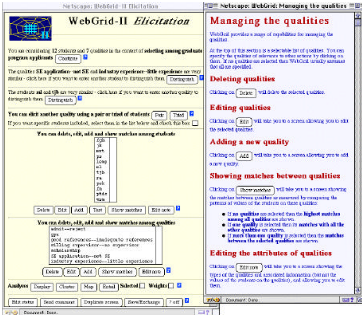
Figure 4 Context-sensitive supportive information in WebGrid-II
