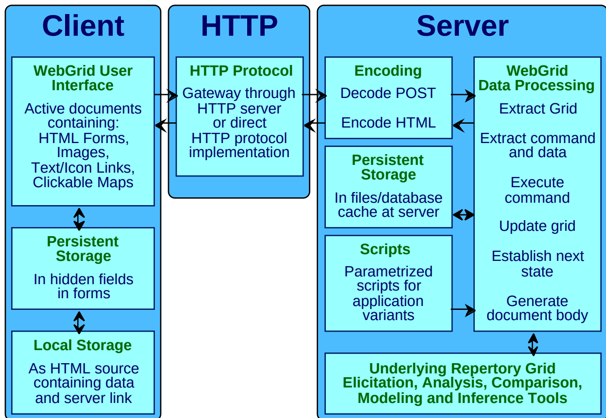
Figure 1 WebGrid-II architecture
