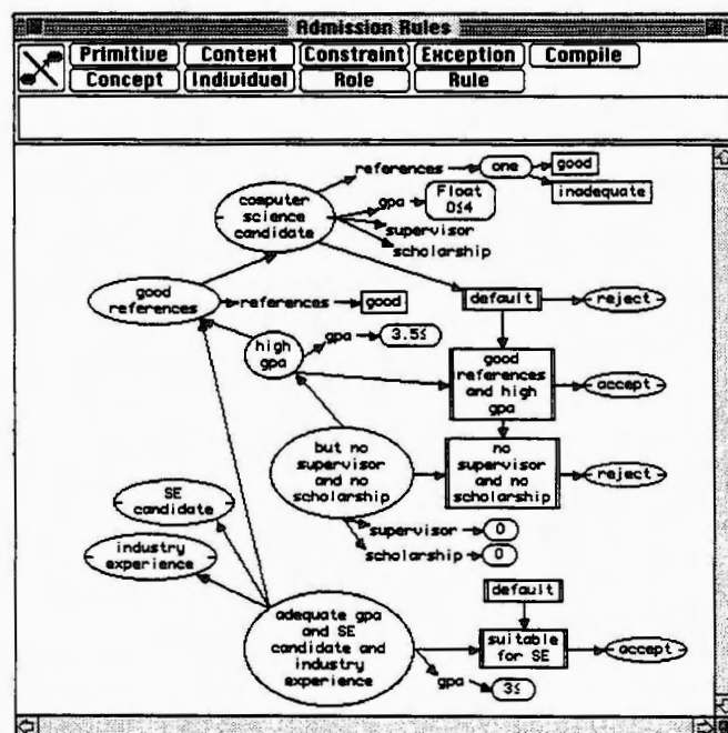
Figure 15 Final rules with exceptions in KDraw
