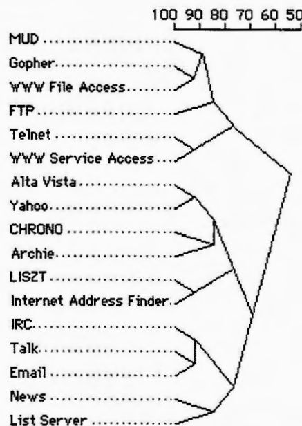
Figure 4 FOCUS reconstructing Internet hierarchy
