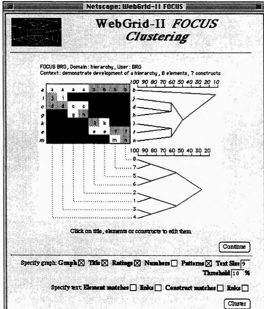
Figure 2 FOCUS reconstructing the hierarchy
