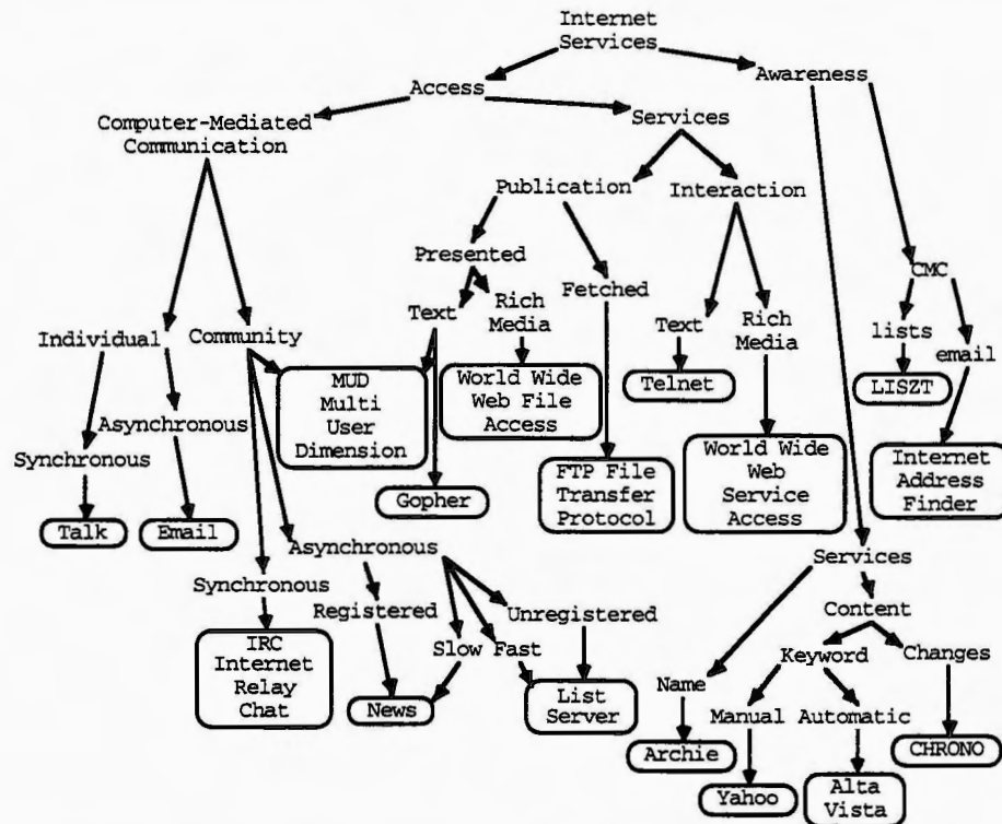
Figure 3 Hierarchy of Internet Services (Gaines et al., 1997)
