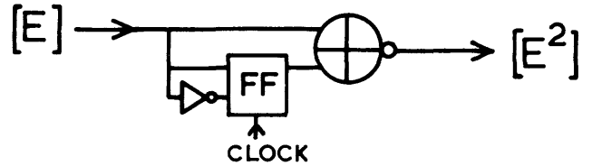
Figure 4—Stochastic squarer
